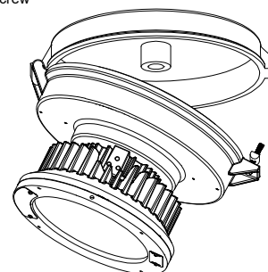
Installation Diagram
